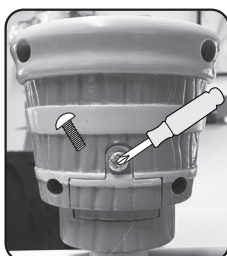
X 3 LR44 BUTTON CELL BATTERIES
